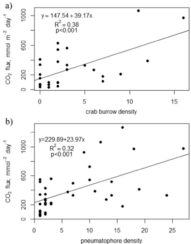
Fig. 5. The relationship between sediment CO 2 flux under dark conditions and the density of (a) crab burrows and (b) pneumatophores in A. marina forests.
