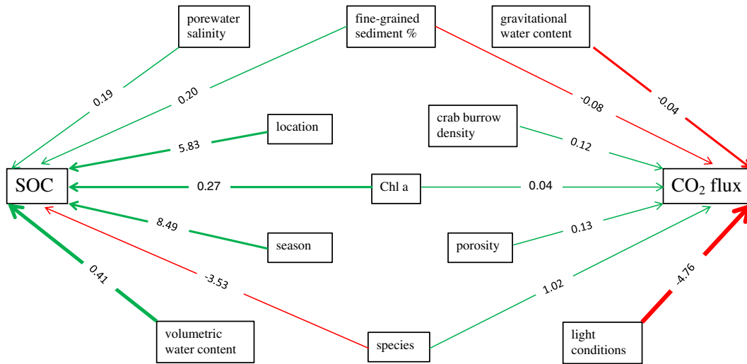
Fig. 4. The final structural equation model. Green and red colours indicate positive and negative estimates, respectively. Numbers in the figure represent each estimate of explanatory variables for SOC or CO 2 flux. The width of the arrows indicates the importance of each estimate.
