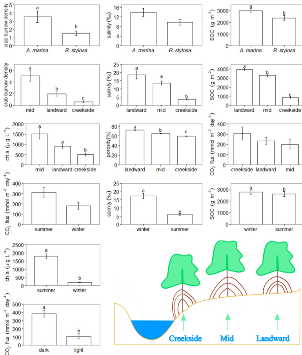
Fig. 3. The difference in sediment CO 2 flux, surface SOC content and physico-chemical properties among seasons, species, light conditions and landform settings. Error bars labelled with different letters were significantly different with each other. For clarity, only Rhizophora is illustrated in the inset on position of the mangrove stands along the creek-land transect.
