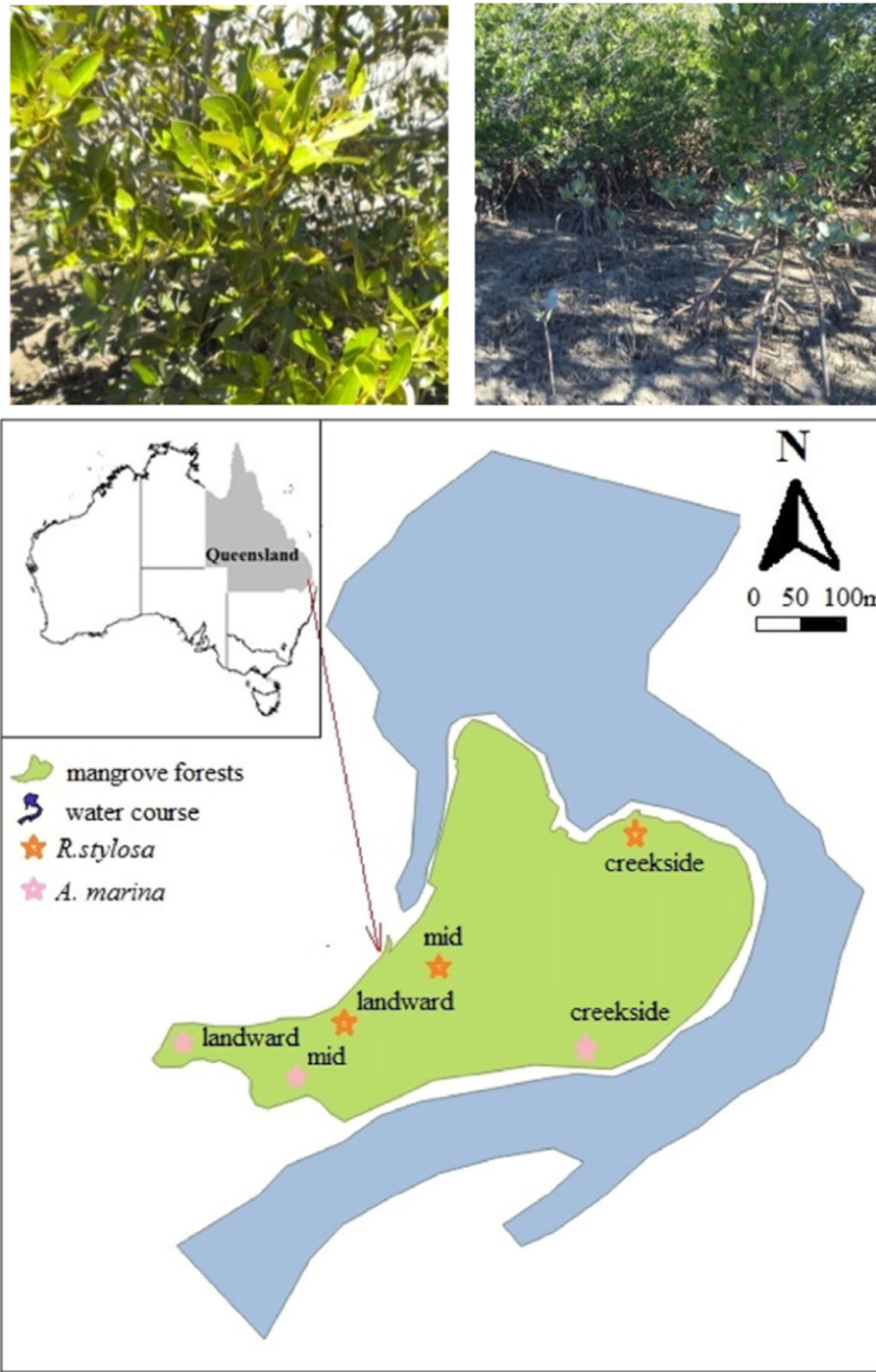
Fig. 2. The sampling location ( 28^{\circ}06'28.8''\text{S} , 153^{\circ}26'48.72''\text{E} ) in Southeast Queensland, Australia. The coordinates of the transects are as below: (1) A. marina (creekside: 28^{\circ}6'32.85''\text{S} , 153^{\circ}26'53.56''\text{E} , mid: 28^{\circ}6'33.48''\text{S} , 153^{\circ}26'44.21''\text{E} , landward: 28^{\circ}6'33.23''\text{S} , 153^{\circ}26'39.74''\text{E} ), (2) R. stylosa (creekside: 28^{\circ}6'26.65''\text{S} , 153^{\circ}26'53.84''\text{E} , mid: 28^{\circ}6'30.38''\text{S} , 153^{\circ}26'47.35''\text{E} , landward: 28^{\circ}6'32.15''\text{S} , 153^{\circ}26'45.06''\text{E} ).
